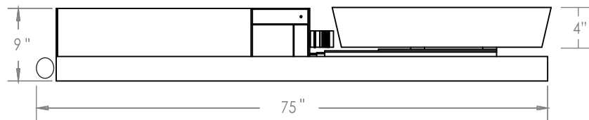
SIDE VIEW- FULLY RETRACTED
