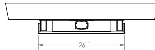
END VIEW- FULLY RETRACTED
