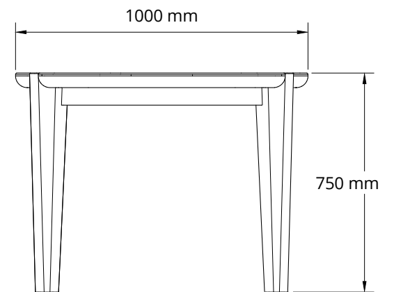
TAMPAK SAMPING
