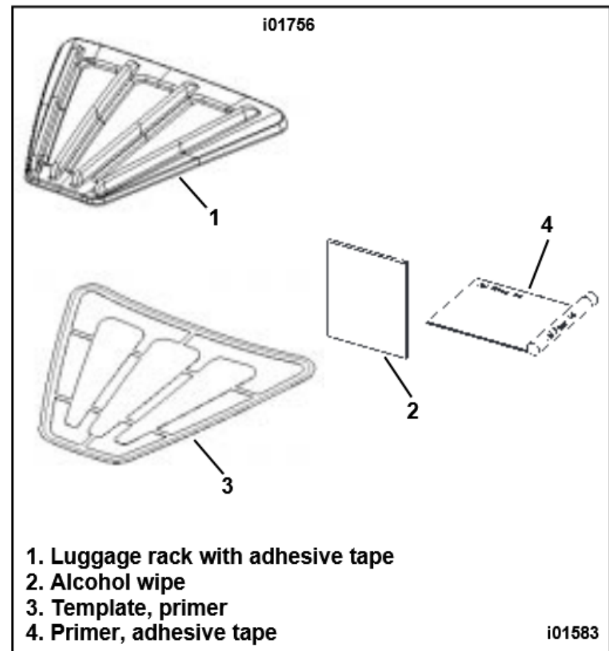
Figure 1. Luggage Rack Kit
