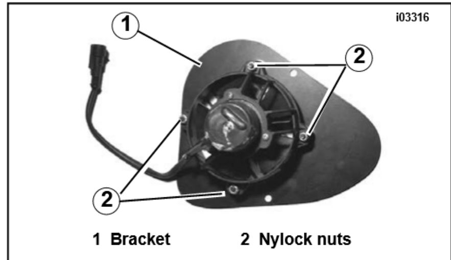
Figure 1. Install Fan Bracket
