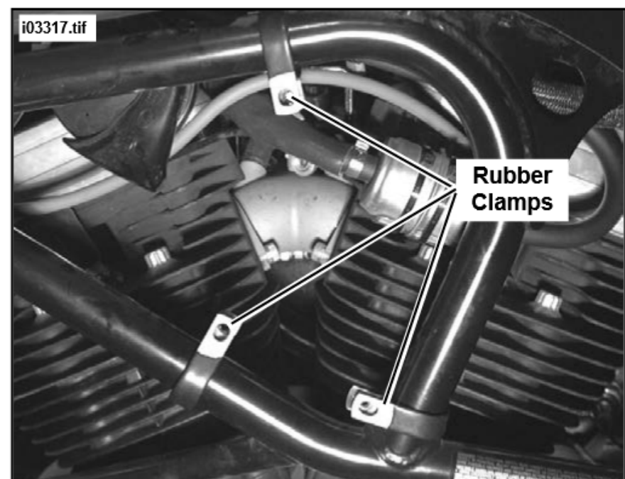
Figure 2. Install Clamps to Frame
