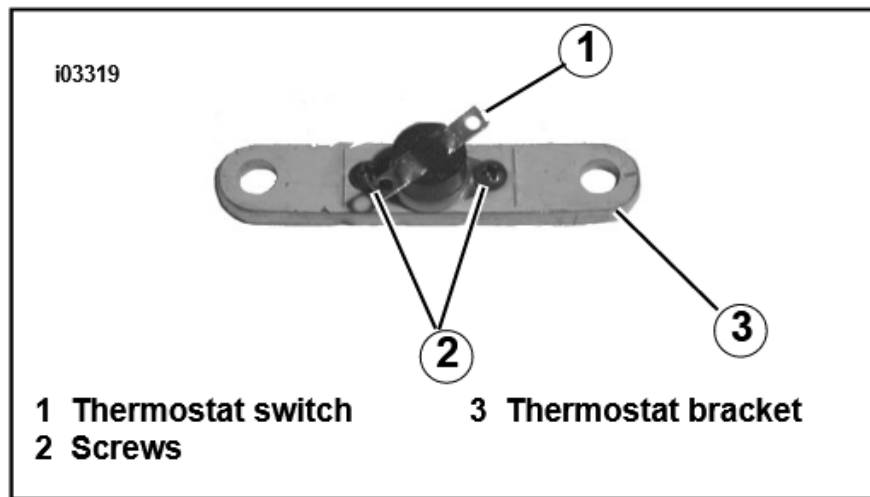
Figure 4. Install Switch to Thermostat Bracket
