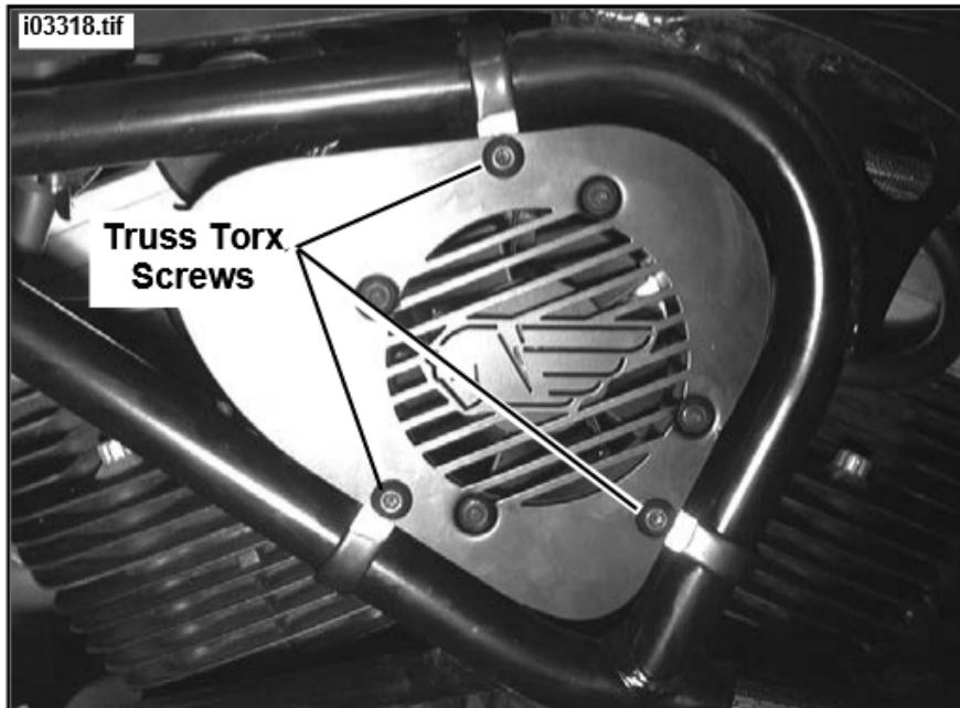
Figure 3. Install Fan Assembly to Frame Brackets
