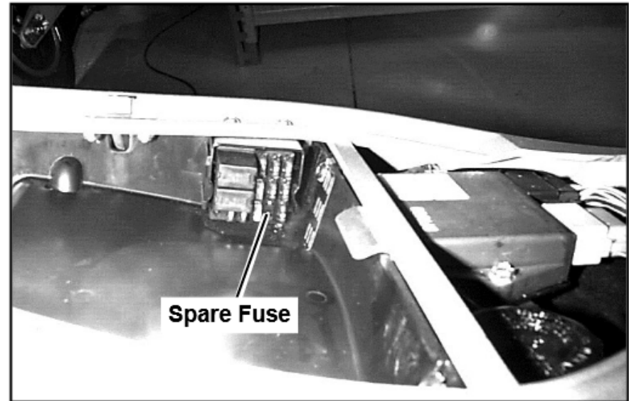
Figure 12. Install Spare Fuse (Motorcycle Trunk)
