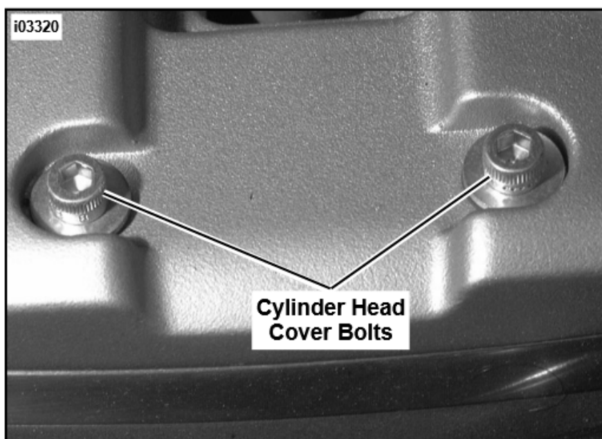
Figure 5. Remove Front Cylinder Head Cover bolts
