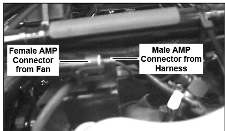
Figure 8. Connect Harness to Fan
