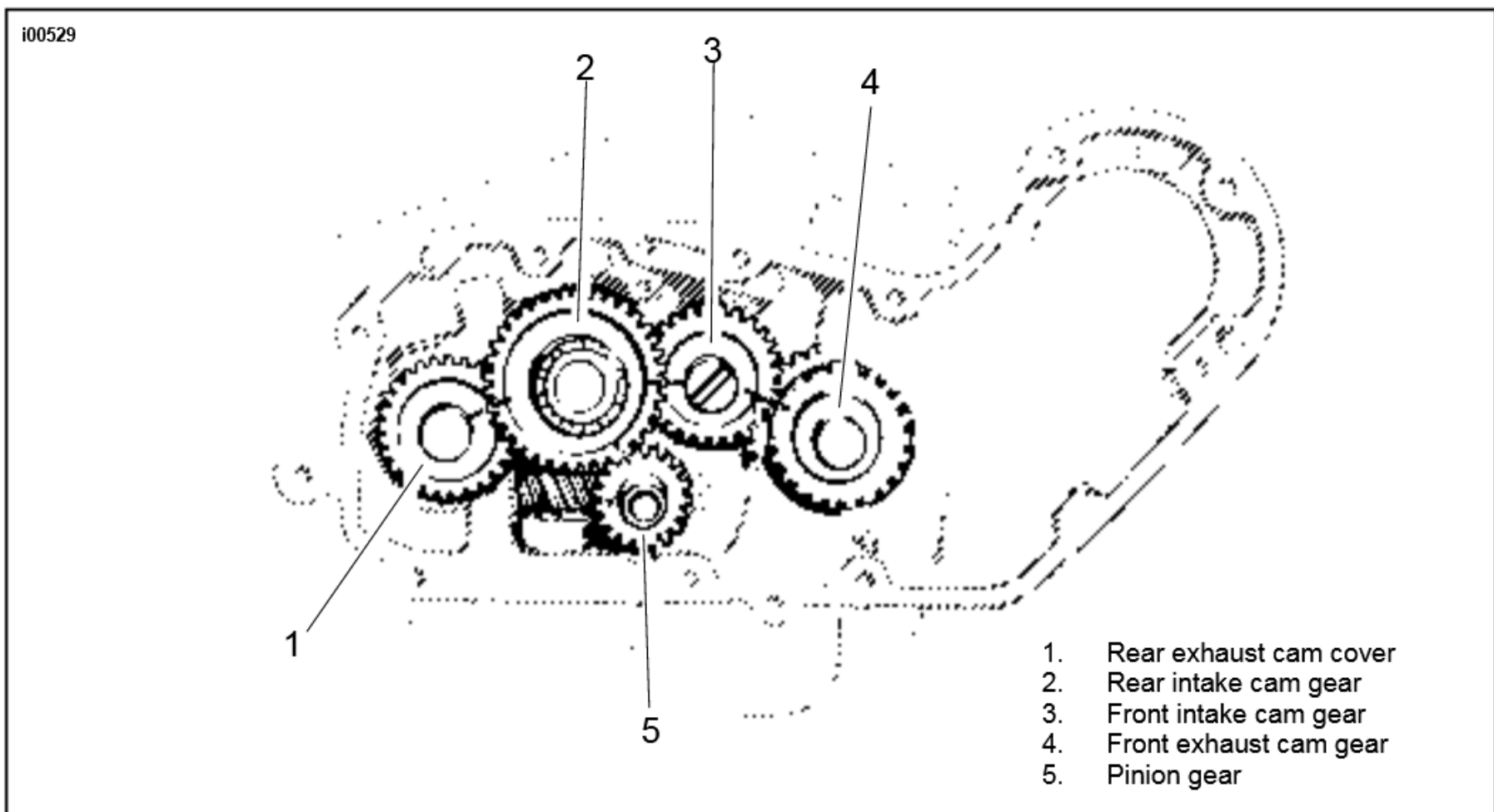
Figure 1. Timing Mark Alignment
