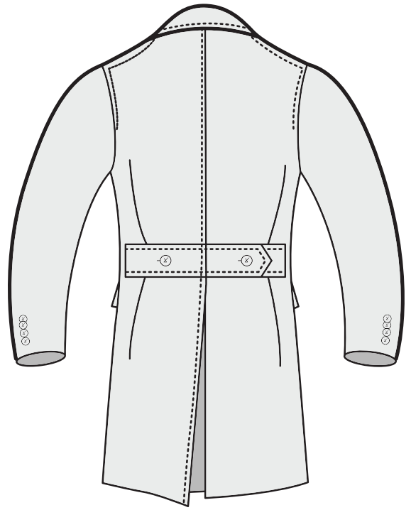
Martingale
