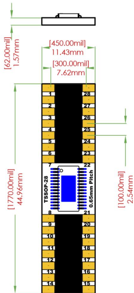
BREAKOUT BOARD DIMENSIONS
