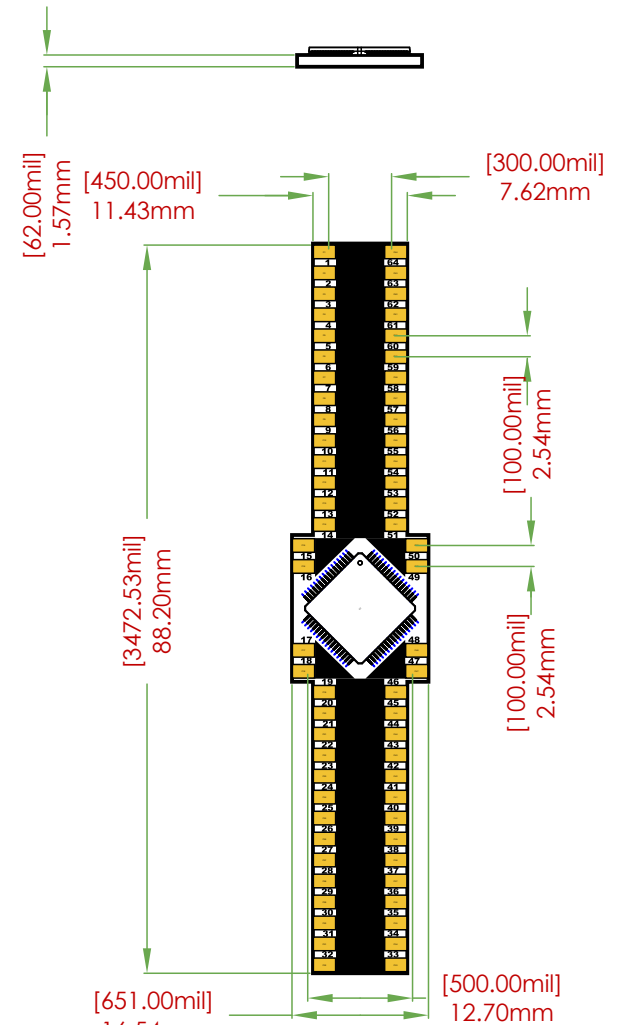
BREAKOUT BOARD DIMENSIONS
