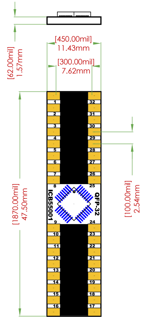
BREAKOUT BOARD DIMENSIONS
