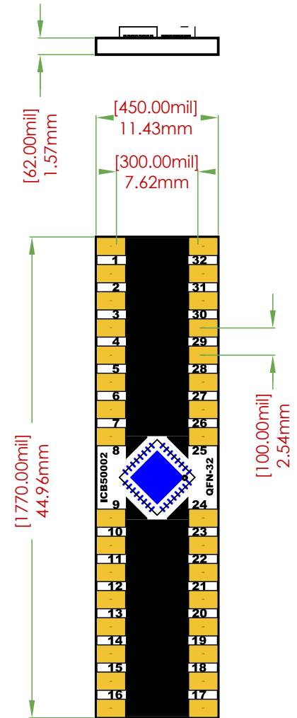
BREAKOUT BOARD DIMENSIONS
