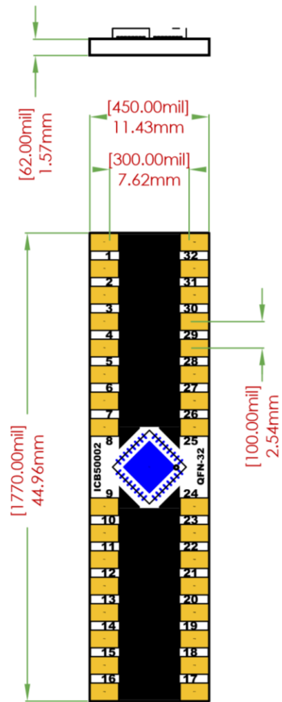
BREAKOUT BOARD DIMENSIONS
