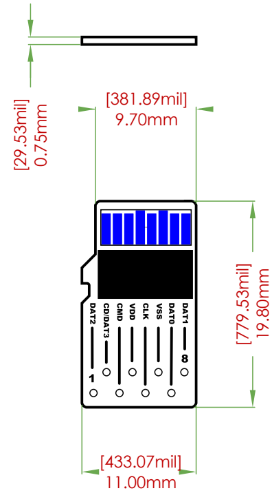
BREAKOUT BOARD DIMENSIONS
