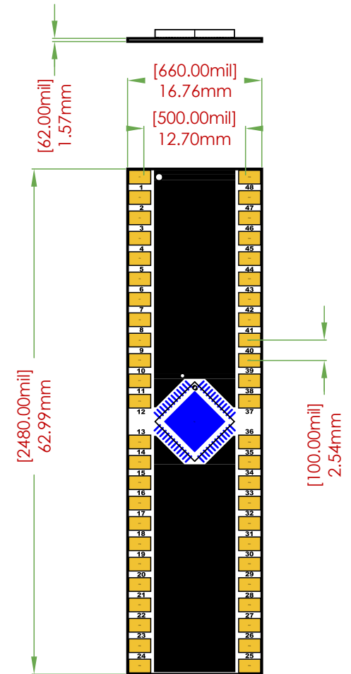
BREAKOUT BOARD DIMENSIONS
