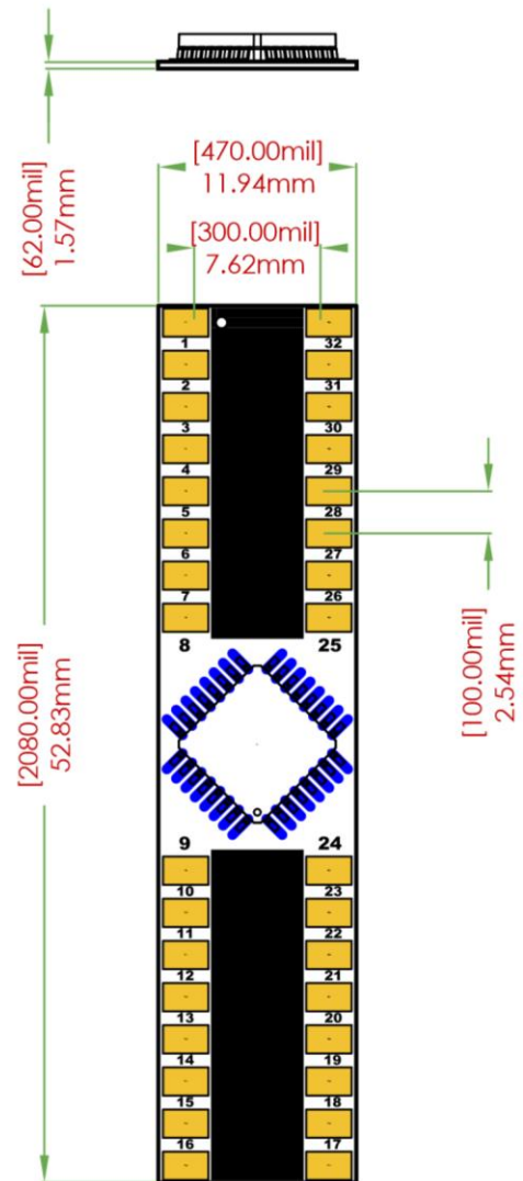
BREAKOUT BOARD DIMENSIONS
