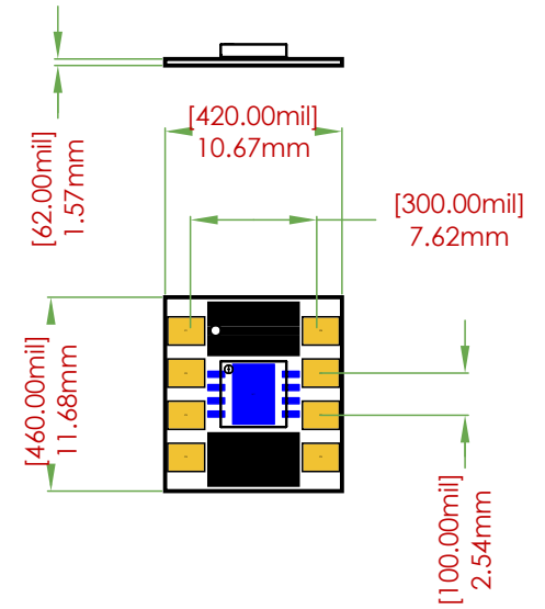
BREAKOUT BOARD DIMENSIONS
