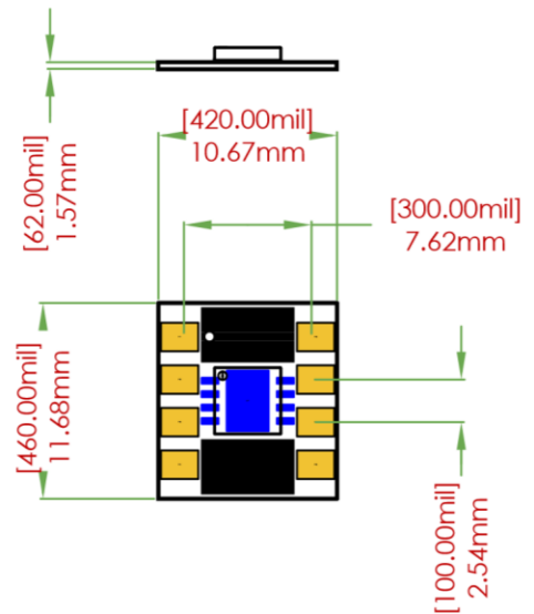
BREAKOUT BOARD DIMENSIONS
