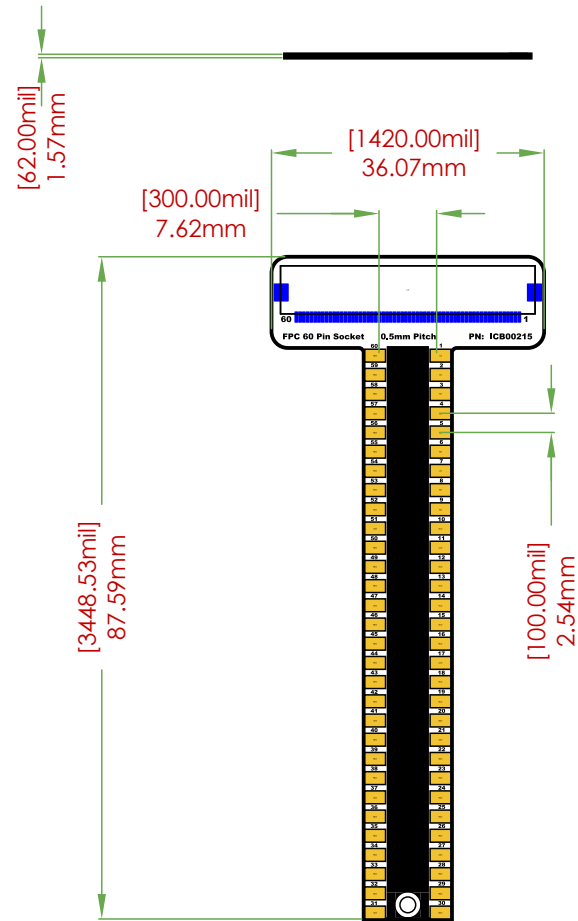
BREAKOUT BOARD DIMENSIONS
