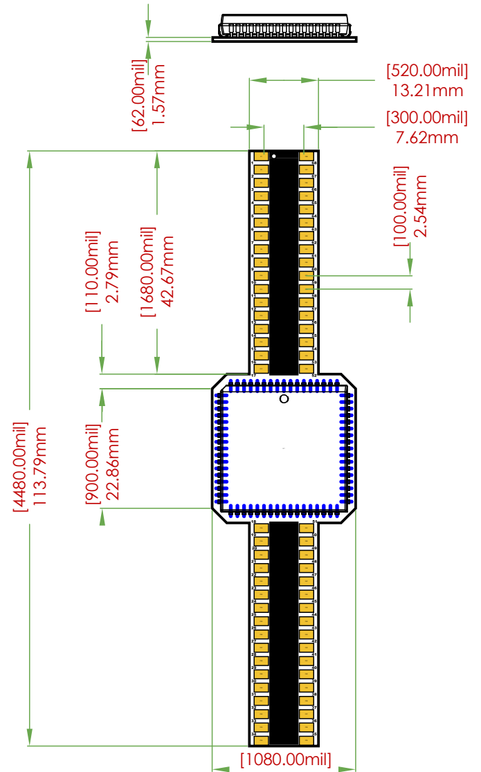
BREAKOUT BOARD DIMENSIONS
