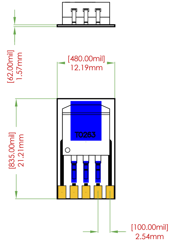
BREAKOUT BOARD DIMENSIONS
