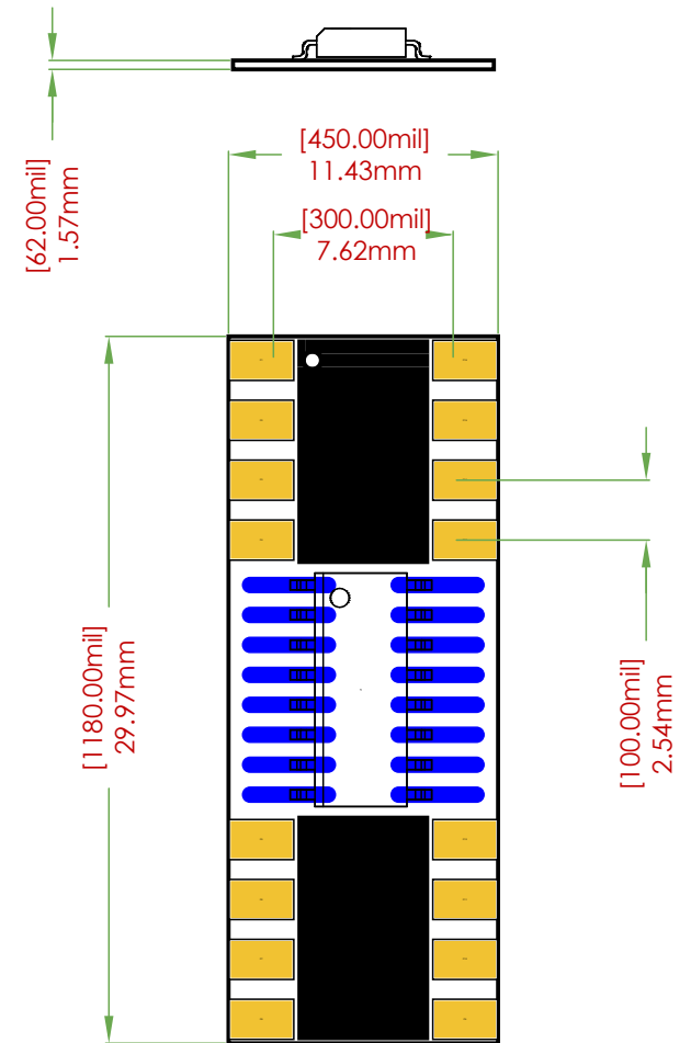
BREAKOUT BOARD DIMENSIONS
