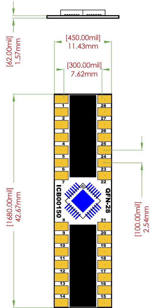
BREAKOUT BOARD DIMENSIONS
