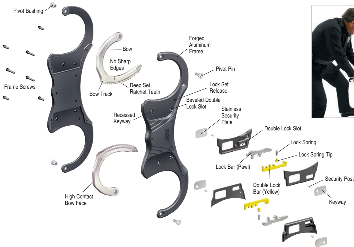
Replaceable Lock Sets are also available in two, three and slip pawl designs.
