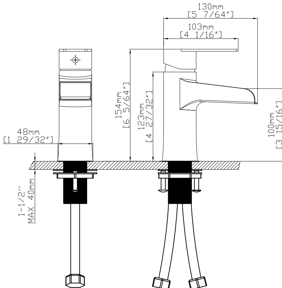
CRITICAL DIMENSIONS
