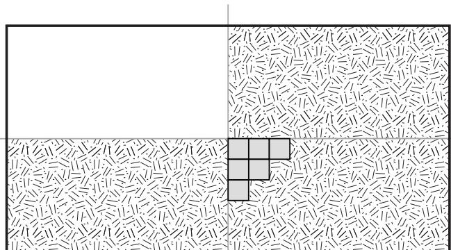
FIGURE 8 Install the field area in a stair step pattern.
