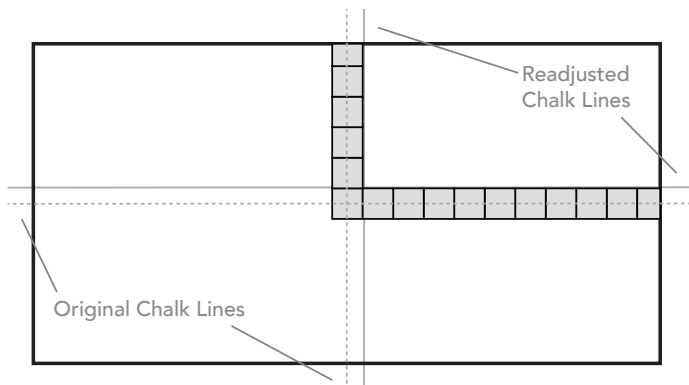
FIGURE 3B: Adjust the layout to eliminate narrow pieces at the ends.
