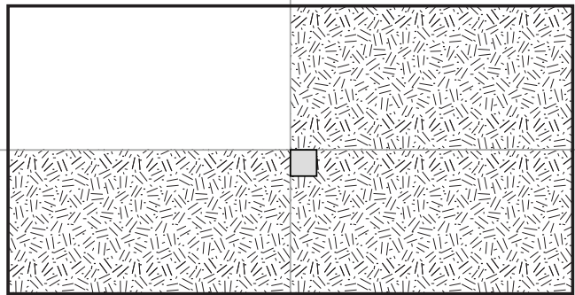
FIGURE 7 Position the tile accurately along the center and perpendicular lines
