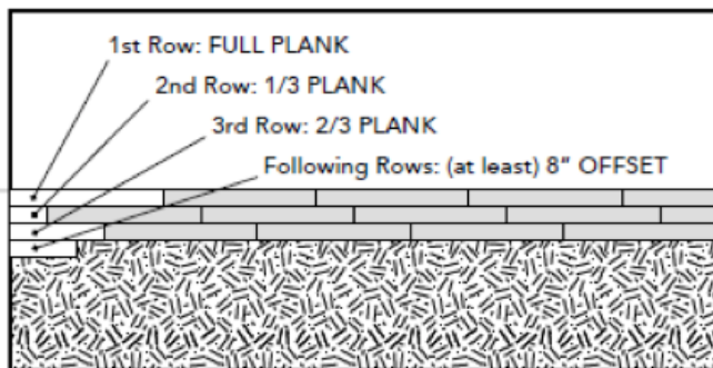
FIGURE 9 Plank layout
