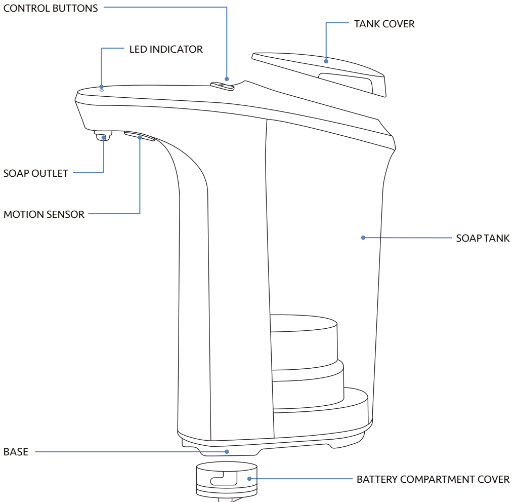
Fig. 1 EXPLODED DIAGRAM
