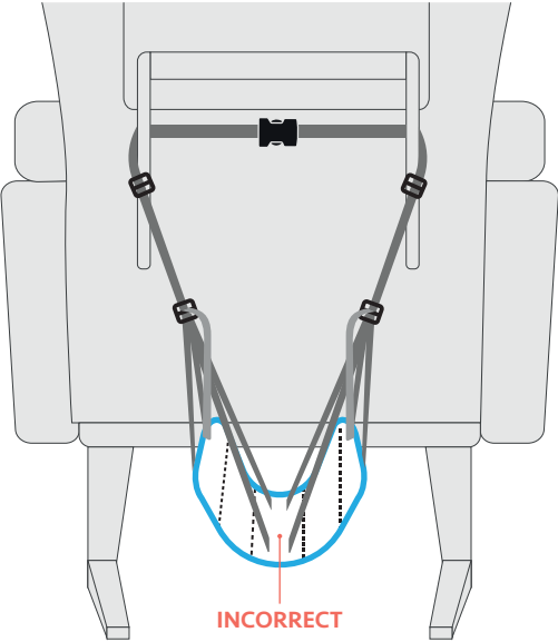
Fig 1. “U” Shape
