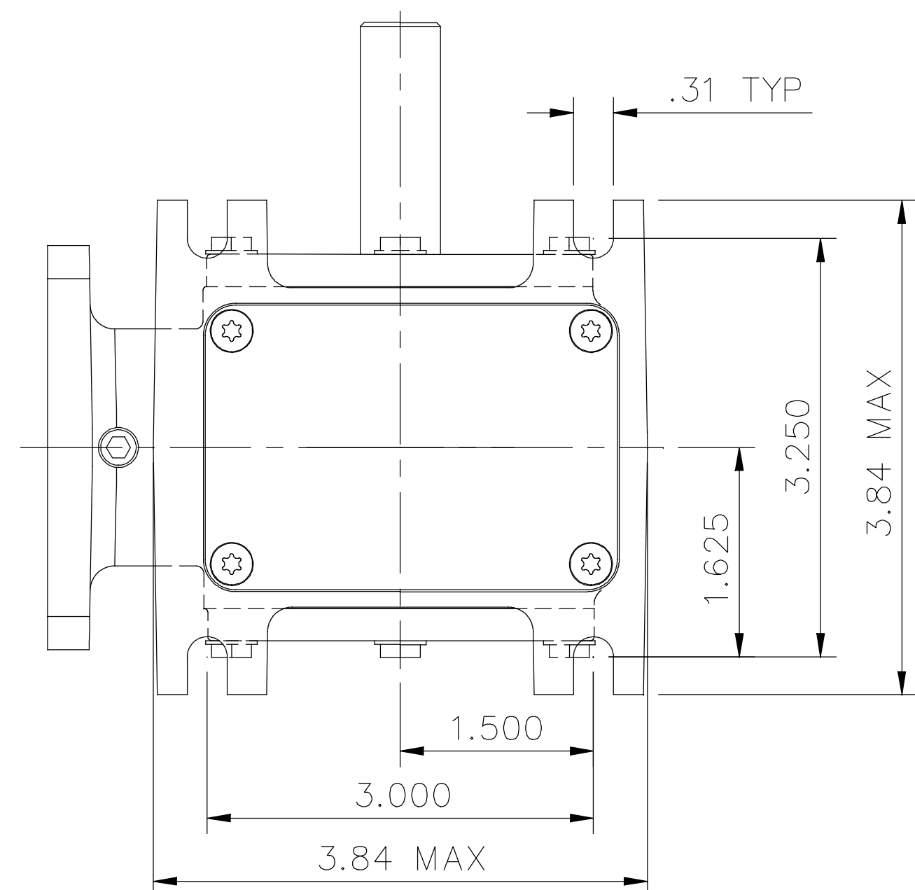
VIEW "Z-Z"
