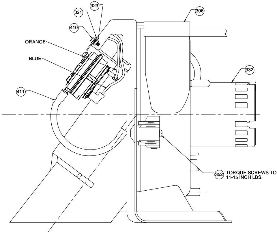
(VIEW WITH COVER INSTALLED)
