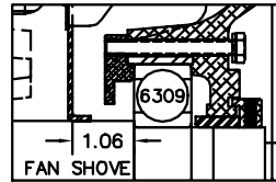
PULLEY END DETAIL
