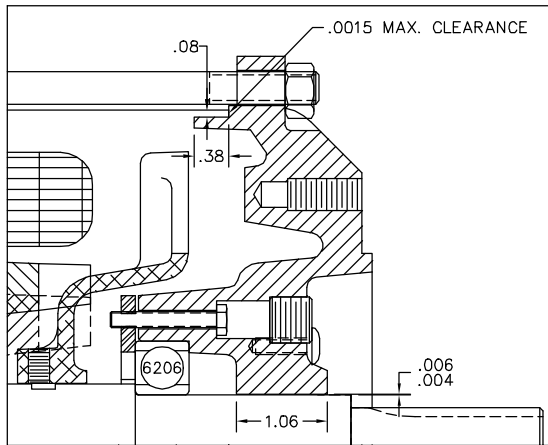
PULLEY END DETAIL
