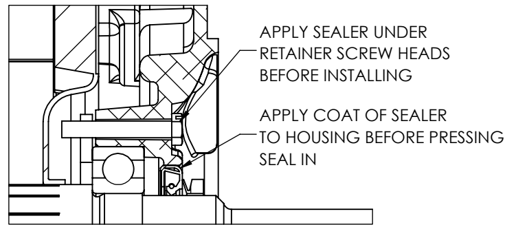
PULLEY END DETAIL
