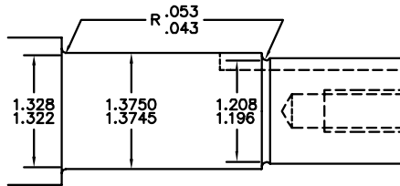
UNDERCUT DETAIL SCALE = .75
