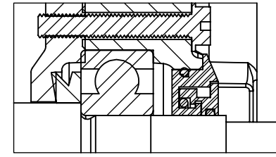
PULLEY END DETAIL
