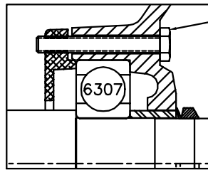
PULLEY END DETAIL
