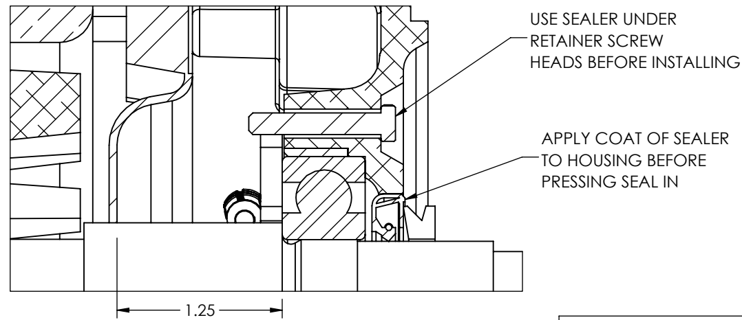
PULLEY END DETAIL
