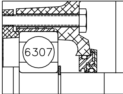
PULLEY END SECTION
