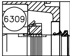
PULLEY END SEAL VIEW
