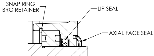
PULLEY END DETAIL
