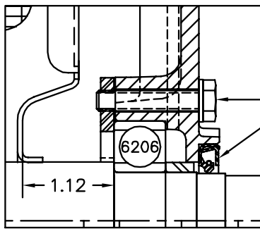
PULLEY END DETAIL
