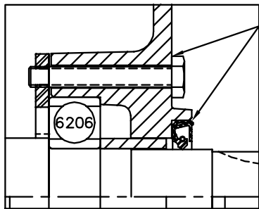
SEAL DETAIL
