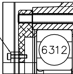
PJ. BRG RETAINER DETAIL
