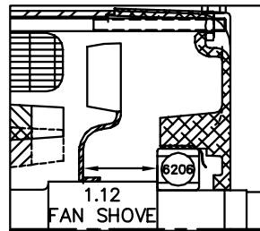
PULLEY END SECTION
