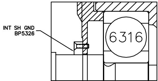
PU_RETAINER DETAIL
