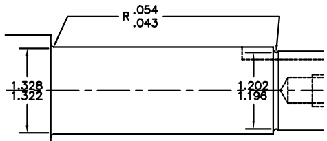
UNDERCUT DETAIL SCALE = .75
