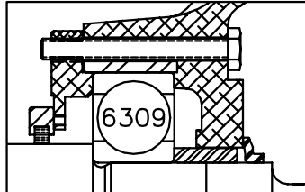
PULLEY END DETAIL
