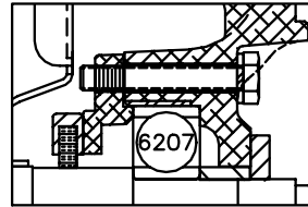
PULLEY END DETAIL (AEGIS GROUND)
