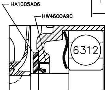
FRONT END DETAIL
