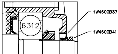
PULLEY END DETAIL
