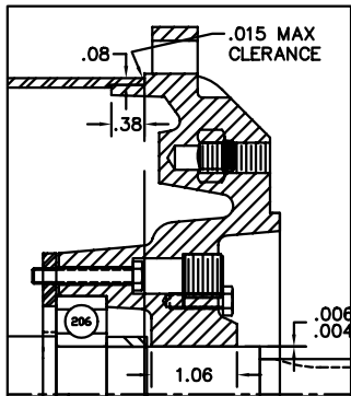
PULLEY END DETAIL
