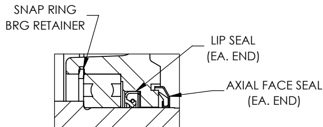
PULLEY END DETAIL
