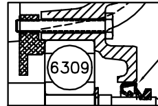
PULLEY END DETAIL
